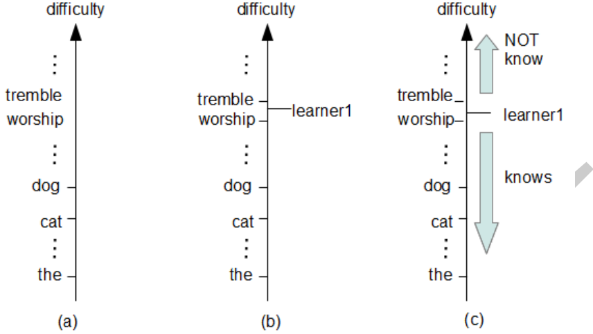
Figure 2: Simple vocabulary prediction model. (a) First, assume there is a difficulty measure that maps each word to a point on the axis of the measure. (b) Second, each learner's ability is also mapped to a point on the same axis. (c) Third, the words with the greatest difficulty to the point designating the learner's ability is predicted to be unfamiliar to the learner, and vice versa.
